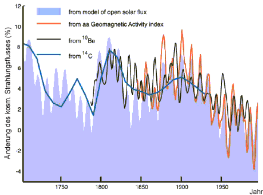
Fig. 2. Change in cosmic ray intensity between 1700 and the present day from four independent proxies. Intensities have been scaled to the 13-GeV cosmic ray data from Huancayo, Hawaii, and then normalized to the 1990–2001 mean. The plot shows deviations from this mean. [Adapted from figure 12 and data in (56)]
